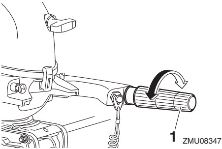
1. Throttle grip
